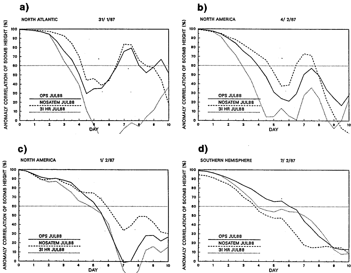
Fig.15 500 hPa height anomaly correlation for limited areas for the four following case studies. Full line: OPS-Jul88 (NESDIS), dashed line: NoSATEM, dotted line: 3I(HR). a) Forecast from 870131-12 UTC North Atlantic, b) 870204-12 UTC North America, c) 870201-12 UTC North America and d) 870207-12 UTC Southern Hemisphere.
