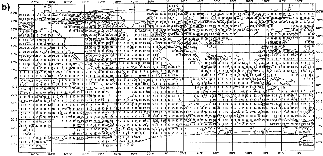
Fig.5 15-day statistics of observed deviations from first-guess stability, T(1000/700)-T(500/300) for 3I soundings, accumulated in 5 \times 5^\circ boxes. a) bias for NOAA-10 clear soundings and b) standard deviation. c) bias for NOAA-10 cloudy soundings and d) standard deviation.
