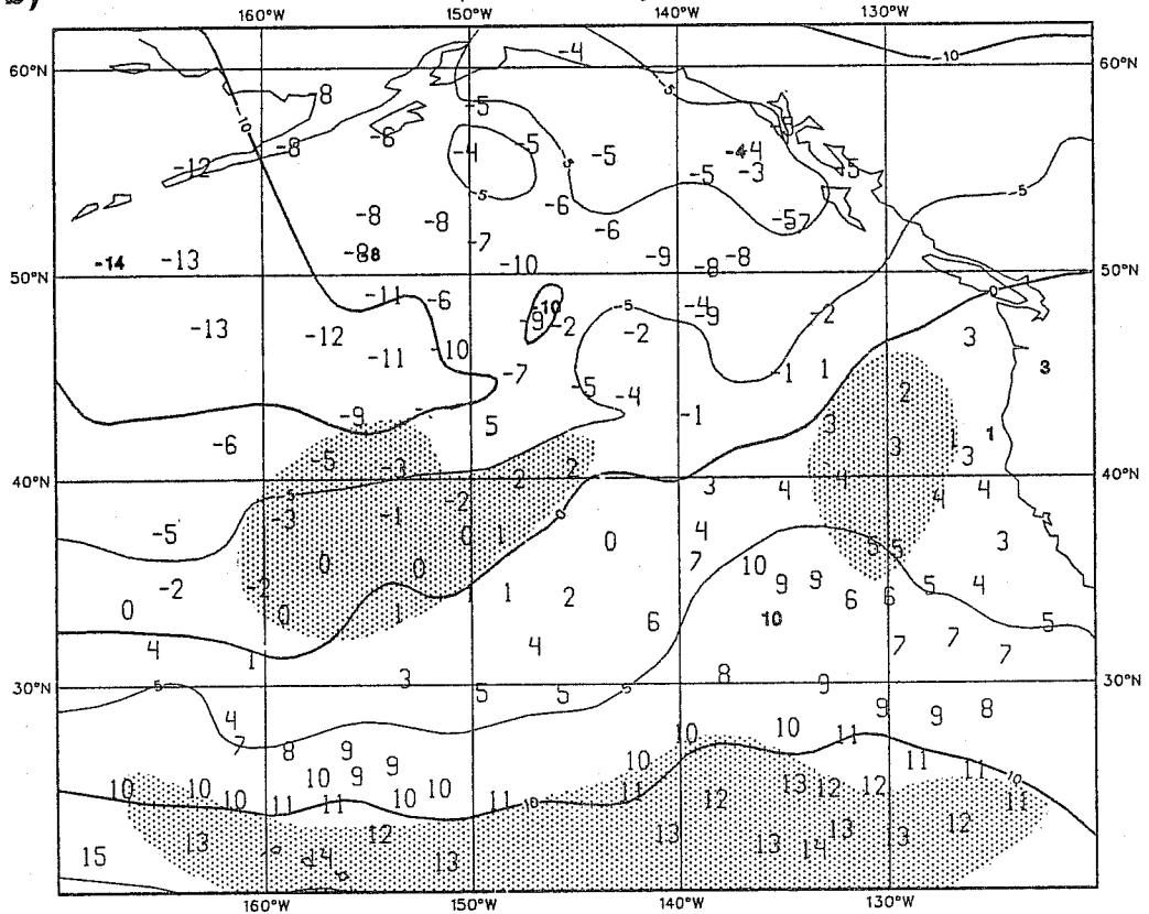
Fig.4 Observed 1000/700 hPa layer mean temperature, 870204-12 UTC in °C. Contour lines are a Cressman analysis of the observed values. a) is 3I, b) is NESDIS. The marked areas are areas with large differences between the two retrieval schemes.
