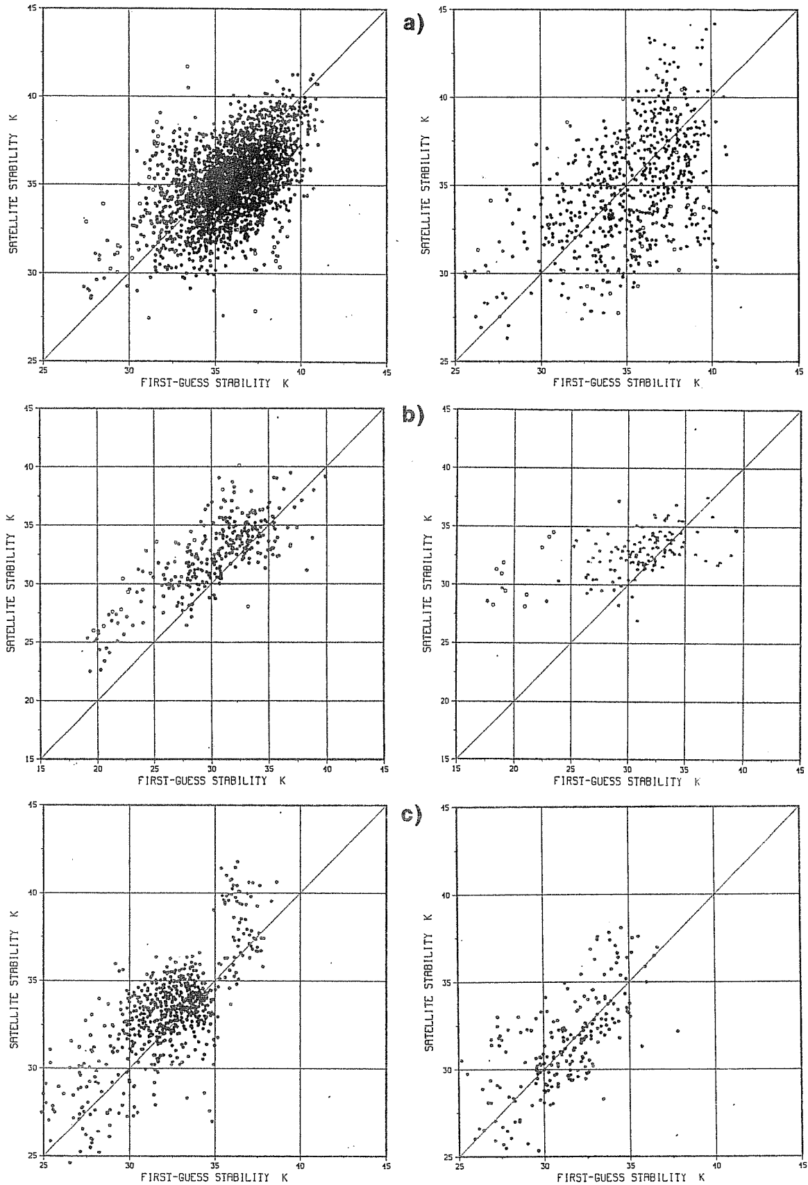
Fig.6 Observed tropospheric stability, T(1000/700) - T(500/300) , retrieved from NOAA-10, versus first-guess stability in ^{\circ}\text{C} , for three different areas, February 1987. 3I to the left and NESDIS to the right. a) North Atlantic ( 50^{\circ}\text{N} - 68^{\circ}\text{N} , 40^{\circ}\text{W} - 5^{\circ}\text{E} ), b) South of Japan ( 25^{\circ}\text{N} - 35^{\circ}\text{N} , 130^{\circ}\text{E} - 140^{\circ}\text{E} ) and c) Midway & Hawaii ( 19^{\circ}\text{N} - 29^{\circ}\text{N} , 180^{\circ}\text{W} - 155^{\circ}\text{W} ).
