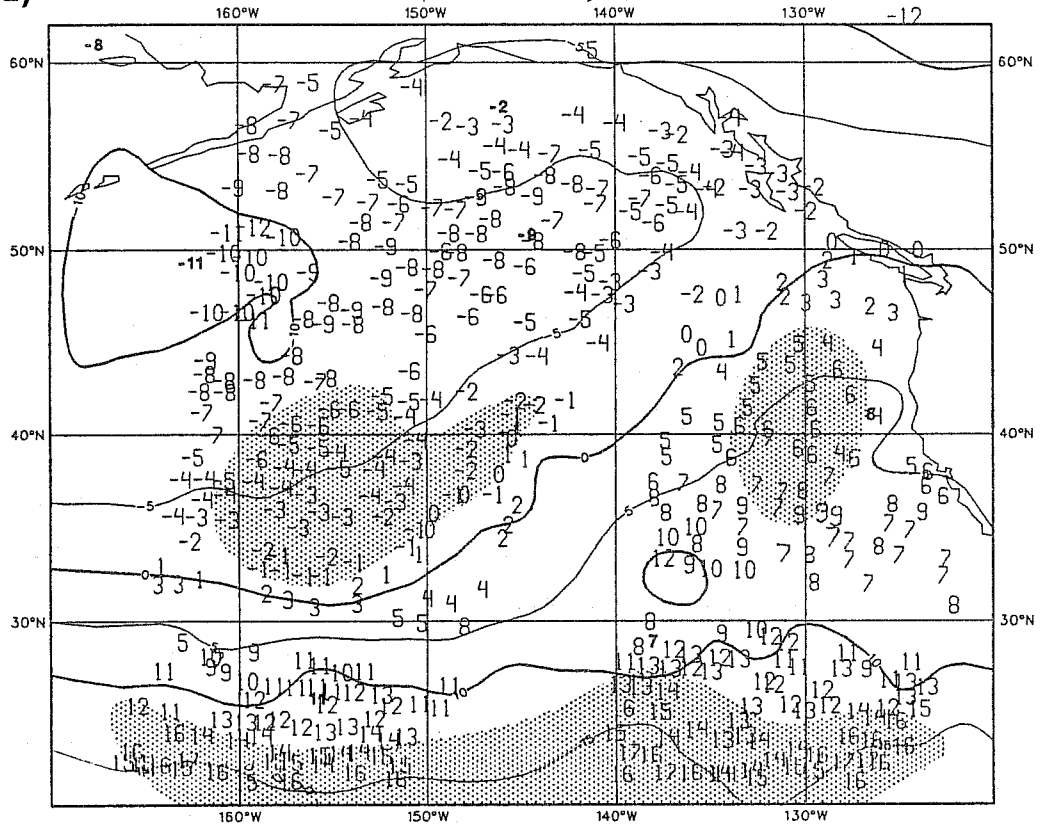
b) 1000 to 700 hPa TOVS Temp retrieved by NESDIS J75 870204-12 UTC
