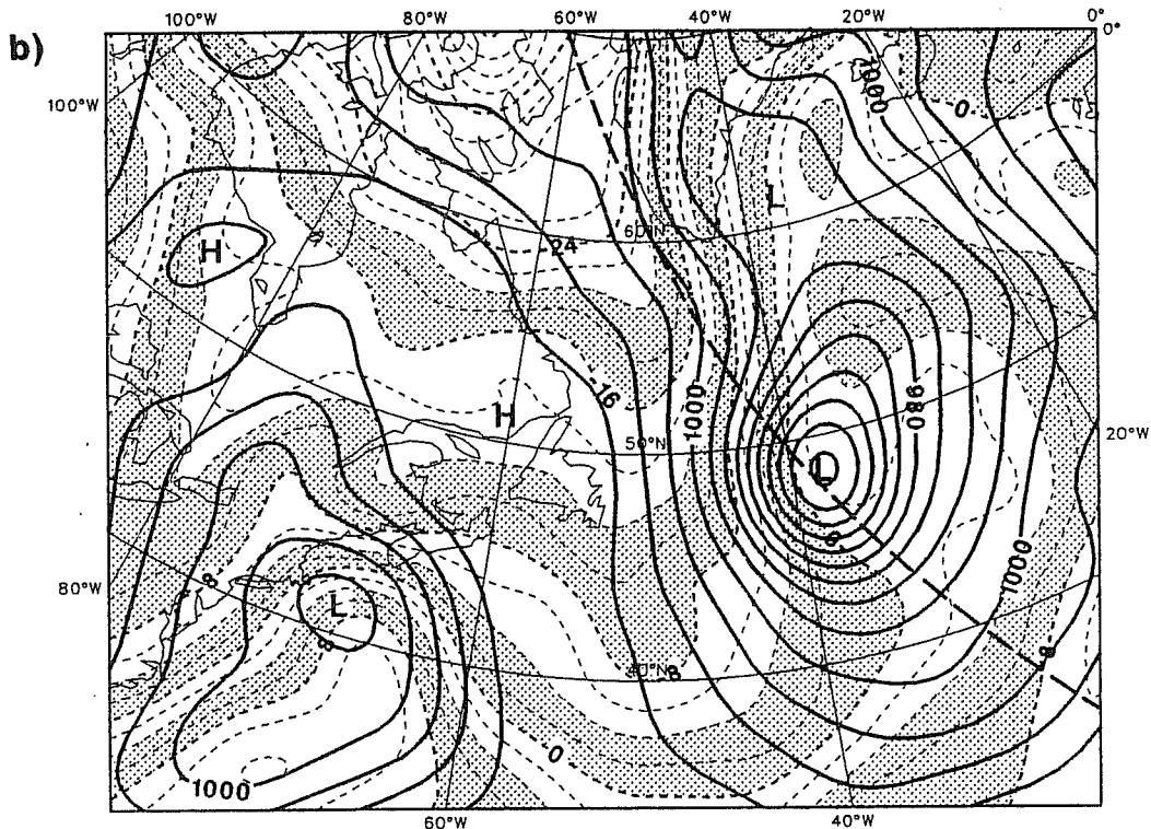
Fig.11 Analysis of mean sea level pressure in hPa, full lines, and 850 hPa temperature, dashed and shaded in intervals of 4°C, for western North Atlantic, 870131-12 UTC. a) is 3I and b) is NoSATEM.
