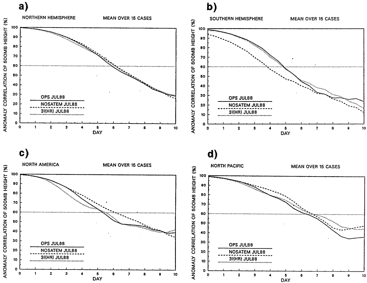
Fig.8. 15-day average of 500 hPa height anomaly correlation for three sets of forecasts. Full line: OPS-Jul88 (NESDIS), dashed line: NoSATEM and dotted line: 3I. a) Northern Hemisphere, b) Southern Hemisphere, c) North America and d) North Pacific.
