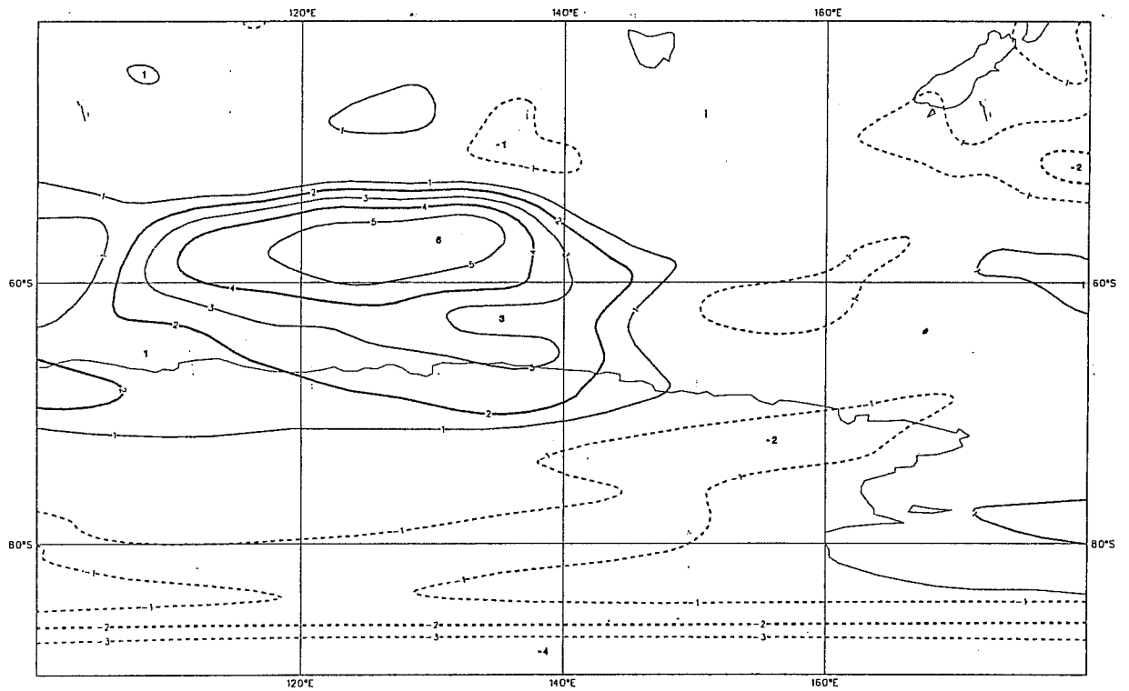
Fig.19 500/300 analysis difference between 3I and OPS-Jul88 (NESDIS) analysis at 870207-12 UTC, in °C, for an area between New Zealand and Antarctica. Full lines are positive and dashed are negative.
