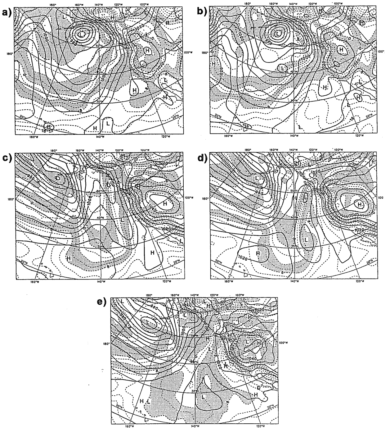
Fig.16 Mean sea level pressure in hPa, full lines, and 850 hPa temperature, dashed and shaded in 4°C intervals, for eastern North Pacific. a) 3I analysis of 870204-12 UTC and b) NoSATEM analysis. c) 3I 2-day forecast from 870204-12 UTC and d) NoSATEM corresponding forecast. e) verifying operational analysis of 870206-12 UTC.
