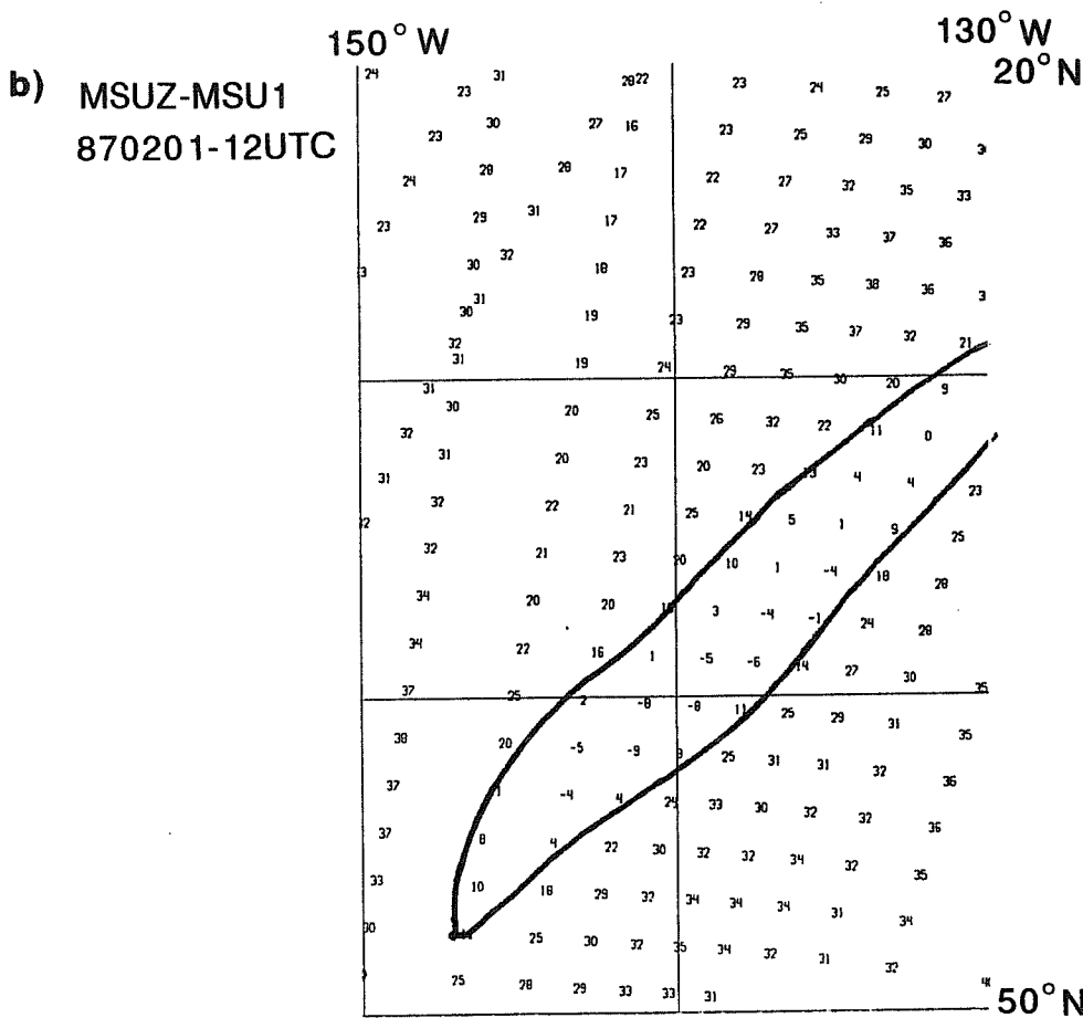
Fig.17 Eastern North Pacific, 870201-12 UTC. a) is observed 1000/500 hPa layer mean temperature deviations from first-guess, in °C. b) is observed MSUZ-MSU1 brightness temperature difference in °C. The 12°C contour line is drawn.
