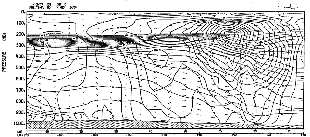
Fig.18 Analysis cross-section from northwest to southeast in eastern North Pacific, along the line marked in Fig. 17a, 870201-12 UTC, showing winds in the plane of the cross-section, arrows, and perpendicular to it, full lines in m/s, as well as potential temperature, thin lines in K. a) is 3I and b) is NoSATEM.
