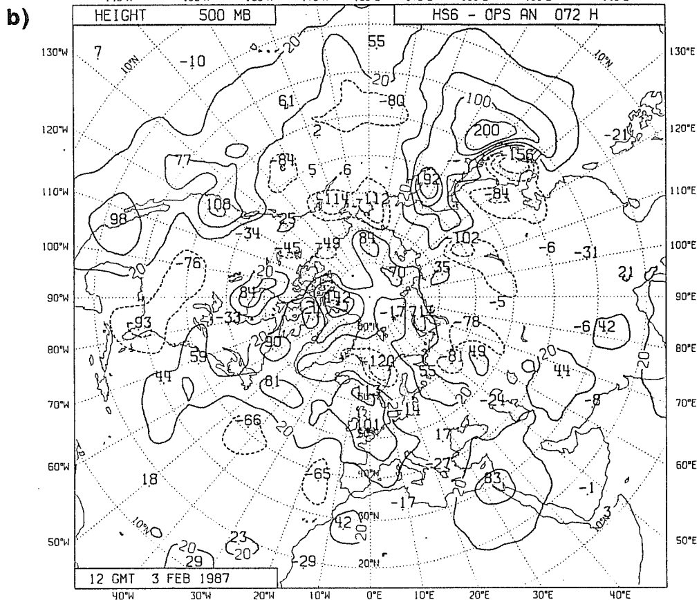
Fig.14 500 hPa 3-day Northern Hemisphere forecast errors of forecast from 870131-12 UTC. Contours are -60, -20 (dashed), +20, +60 (full lines) in metres. Verifying analysis is the operational analysis from February 1987. a) 31 and b) NoSATEM.
