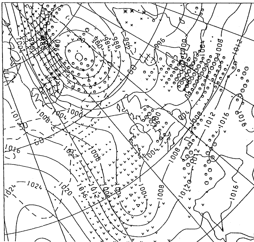
Fig.8. 24 hour PMSL forecast for 00 UTC 21/3/91, previous model.
