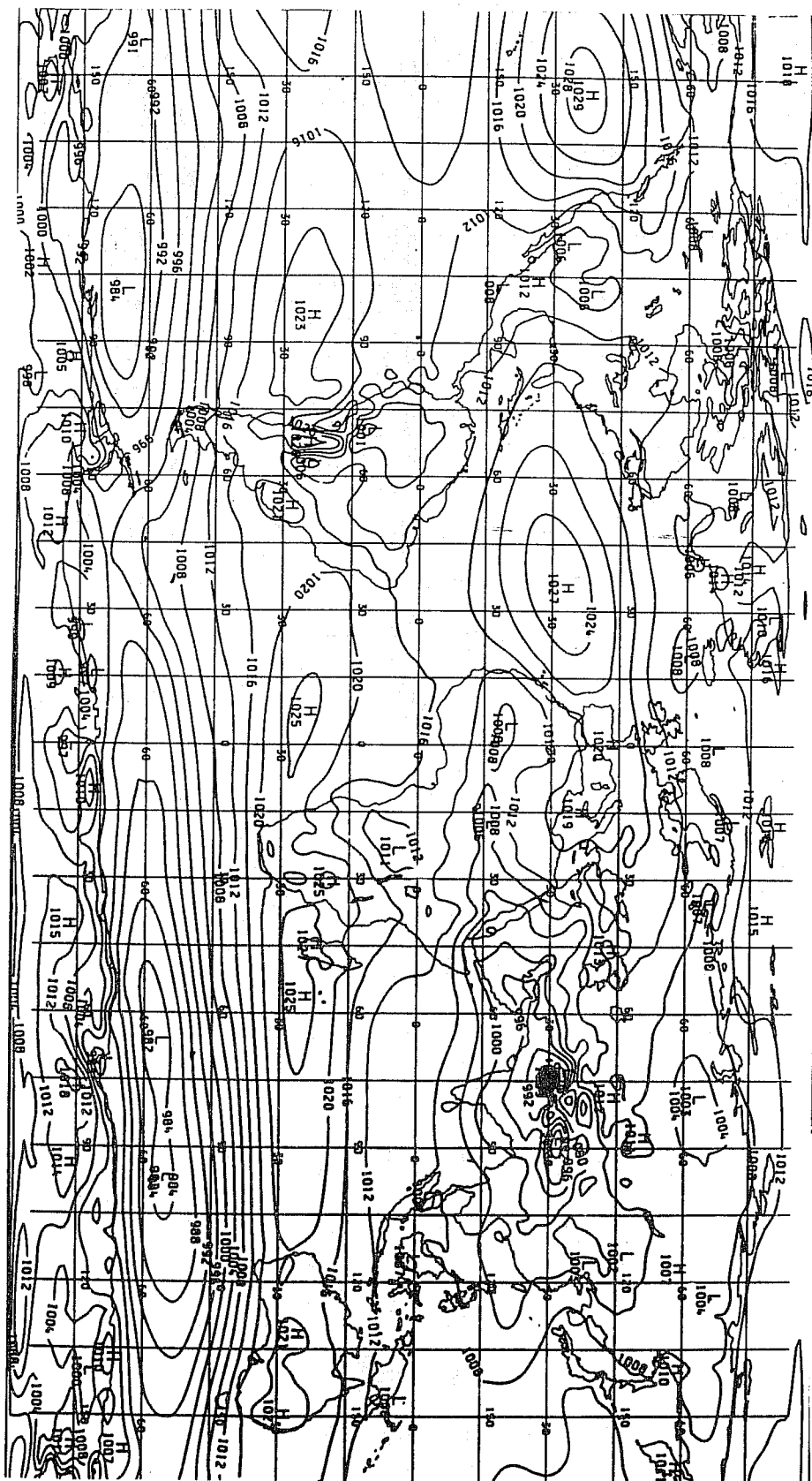
Fig.14. Mean summer (Jun.-Aug.) surface pressure (hpa)from unified model climate simulation.
