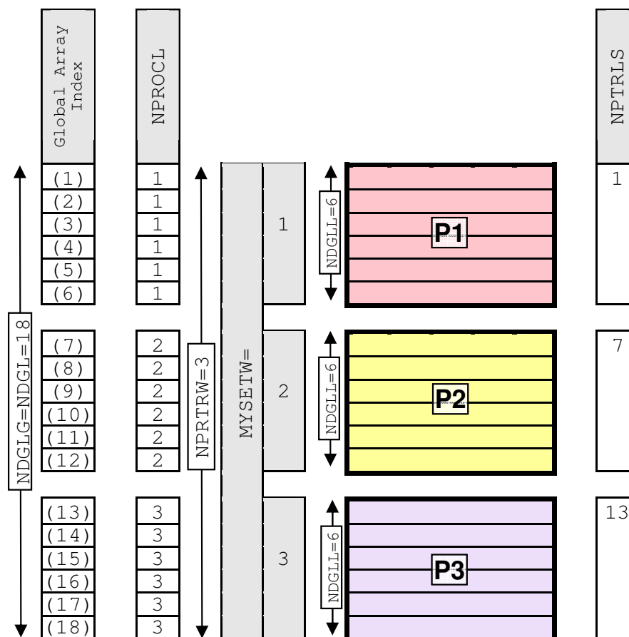
Figure 2.6 Decomposition of zonal waves in Fourier space. Shown here is a single (first) vertical level.
