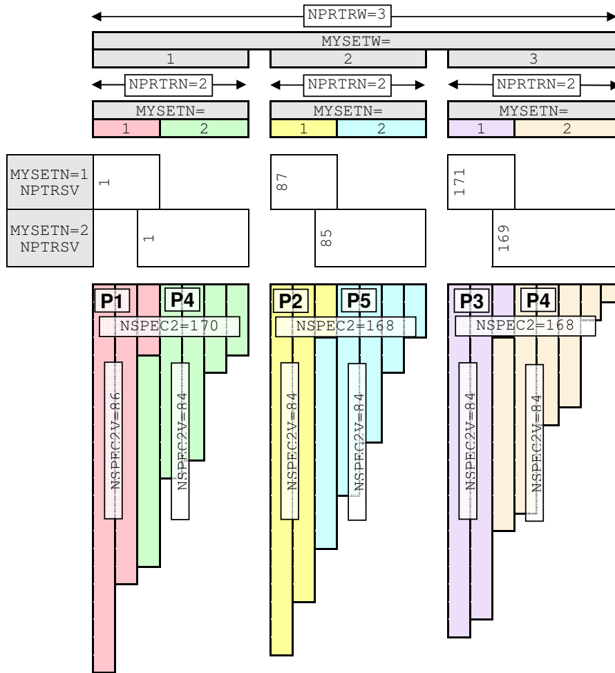
Figure 2.10 Decomposition of spectral data for the semi implicit calculations.
