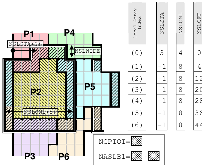
Figure 2.5 The semi-Lagrangian Halo (For processor 2).
