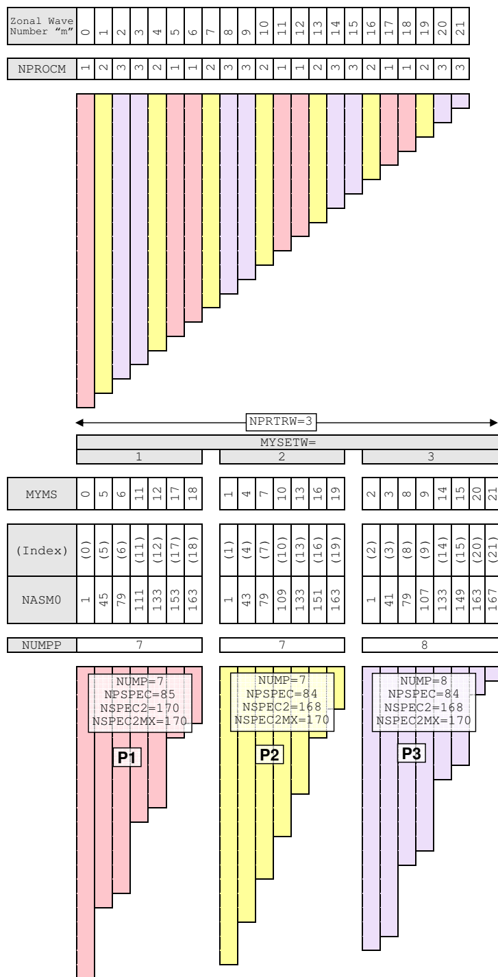
Figure 2.8 Distribution of zonal wave numbers (T21 spectral triangle).
