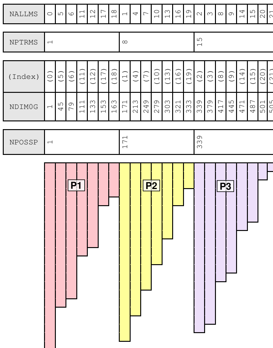
Figure 2.9 Global representation of T21 spectral triangle.
