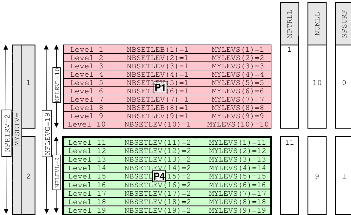
Figure 2.7 Decomposition of vertical levels used in Fourier and spectral space. Shown here is a single “W” set.
