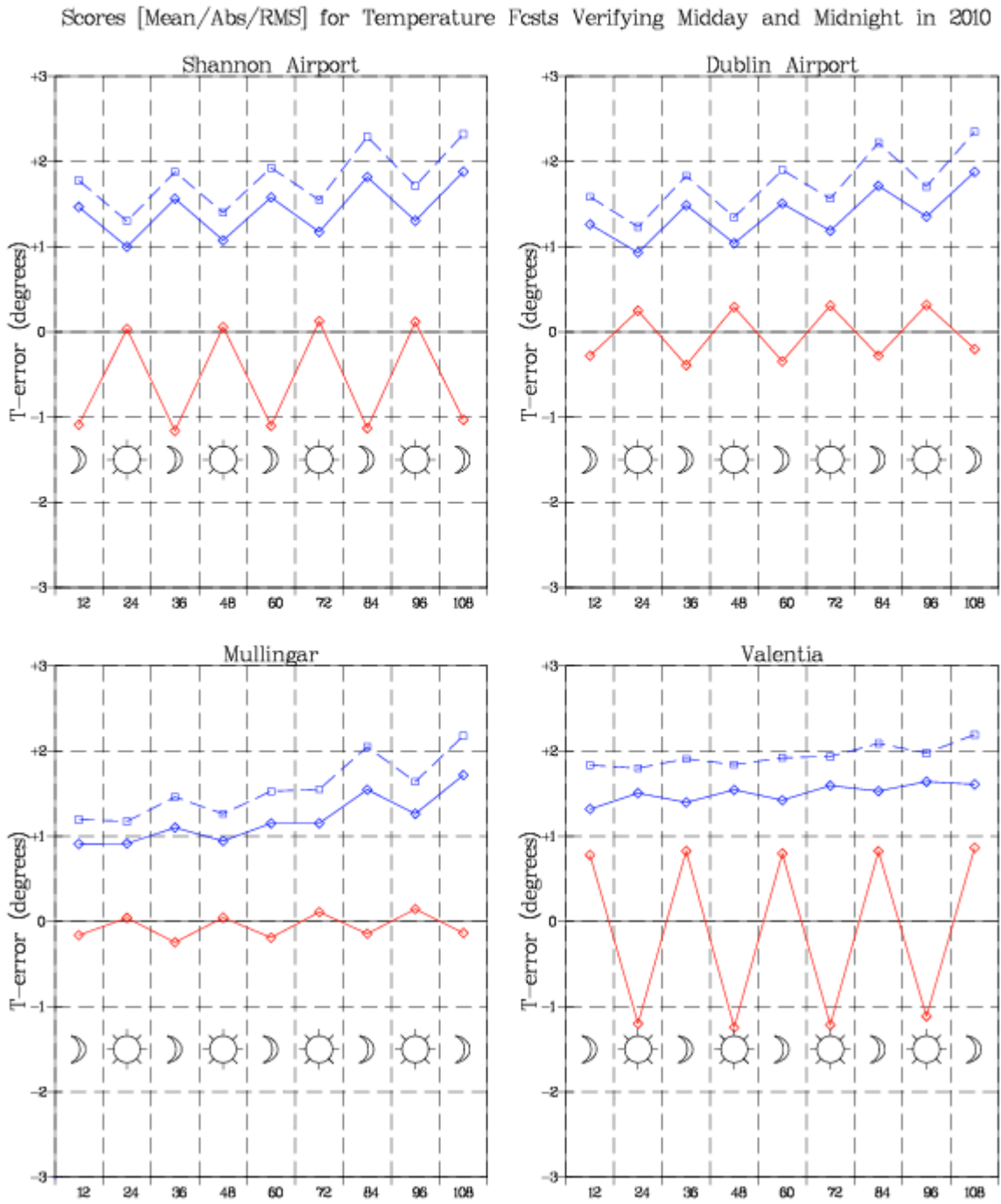
Figure 7 Mean scores for ECMWF forecasts of 2-metre Temperature, in 2010, averaged over a year of data. The solid blue line is the mean absolute error, the dashed blue line the rms error and the red line the mean error or bias. It can be seen that the quality of the forecast decreases with the length of the forecast. The 'sun' and 'moon' symbols indicate forecasts verifying at midday and midnight, respectively. The length of the forecast [in hours] is indicated on the x-axis.
