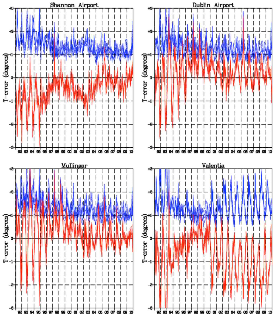
Monthly Scores [Mean/Abs] for Temperature Forecasts Verifying at Midday
