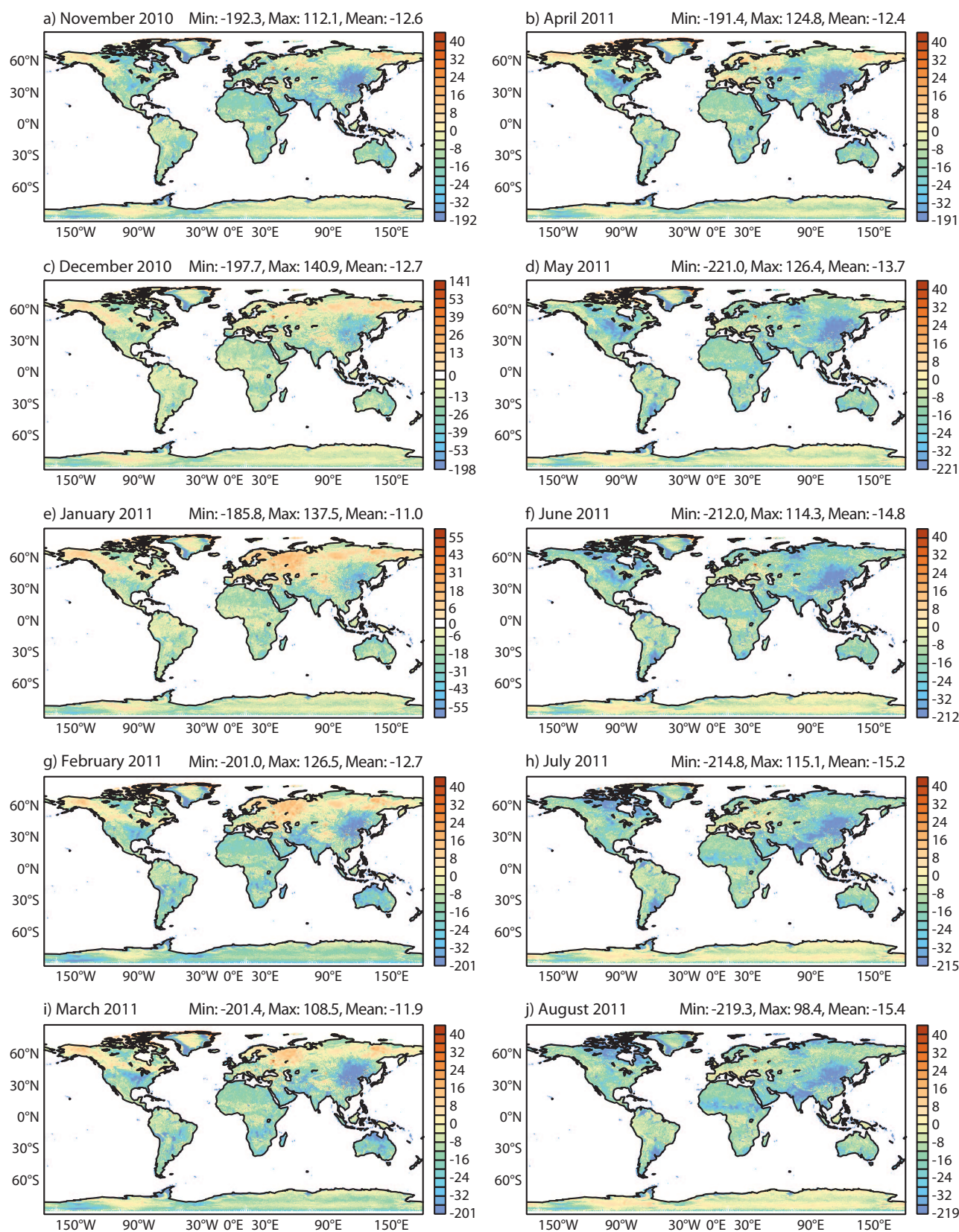
Figure 6: As in Fig. 5, but for YY polarisation.
