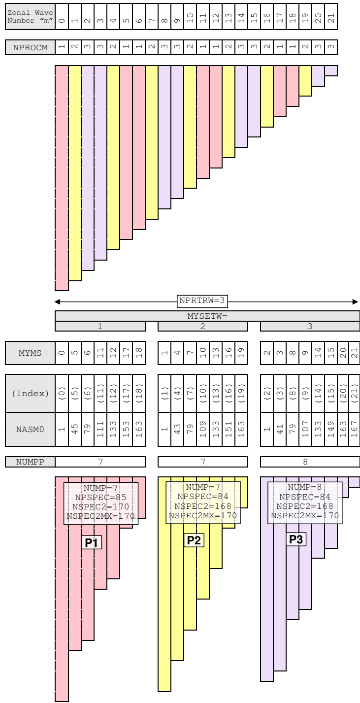
Figure 2.14 Distribution of zonal wave numbers (T21 spectral triangle).
