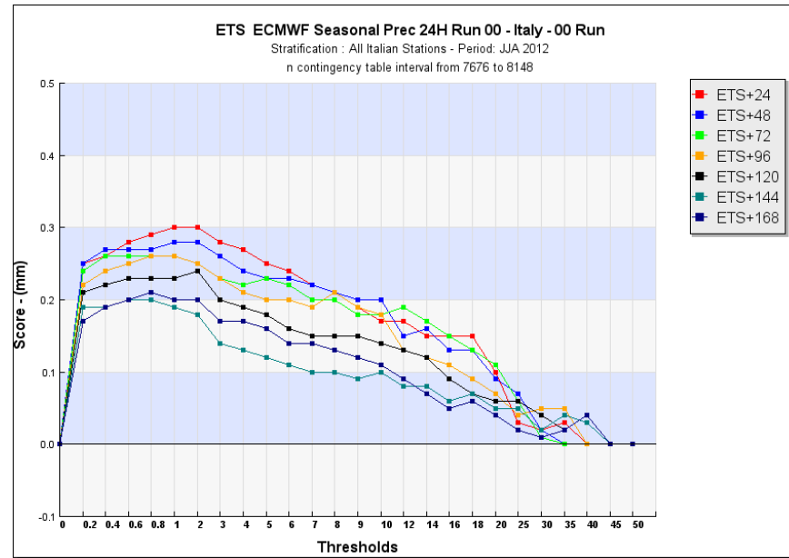
IFS Precipitation in 24 hours - ETS score
