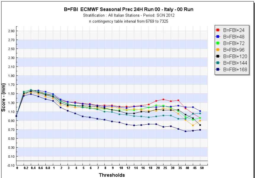
IFS Precipitation in 24 hours - FBI score
