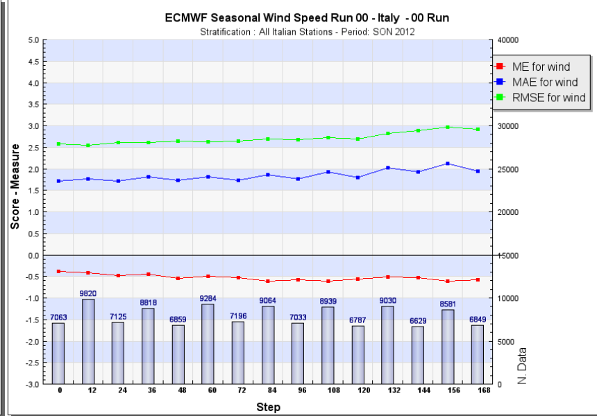
IFS Wind Speed (Mean Absolute Error, Mean Error and Root MSE)
