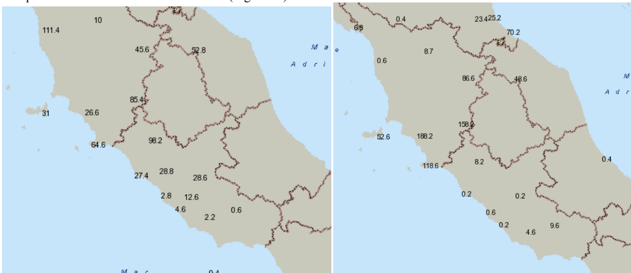
Fig 6 Rainfall Data by AM network (left: 11 th nov 2012 00-24h; right 12th nov 00-24h)
