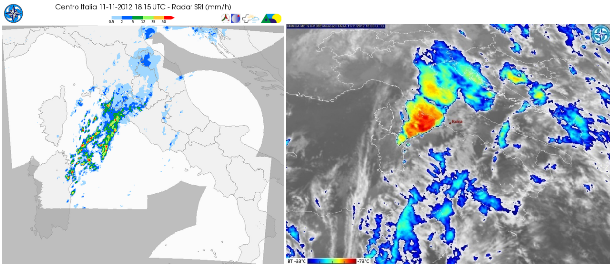
Fig 5 Situation at the time 18 UTC del 11 nov: radar (left) and satellite Met 9 IR Enhanced (right) showing brightness Temperature at clouds top
