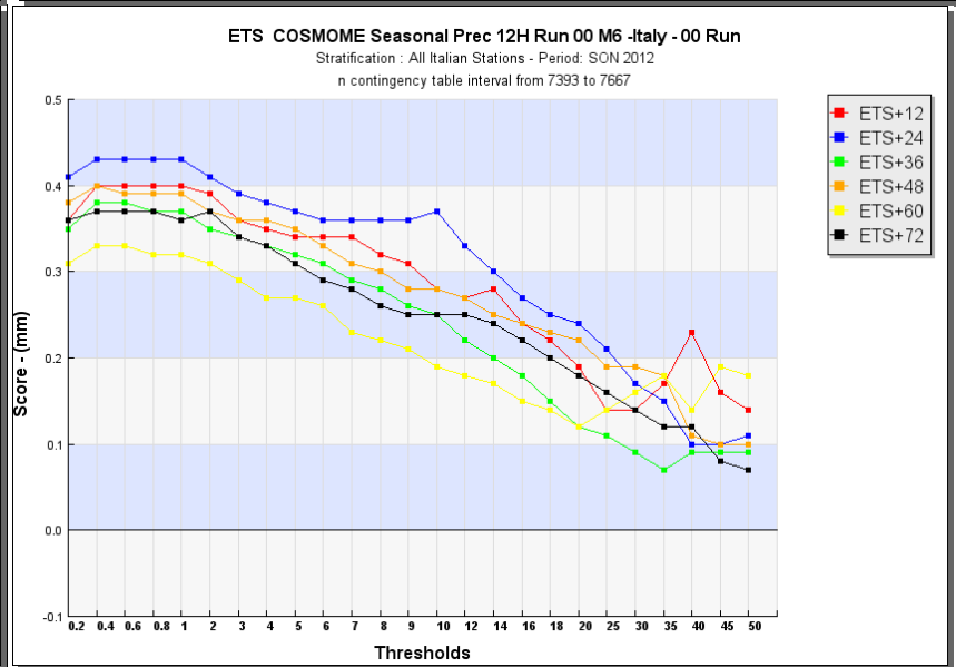
COSMO-ME Precipitation in 12 hours - ETS score
