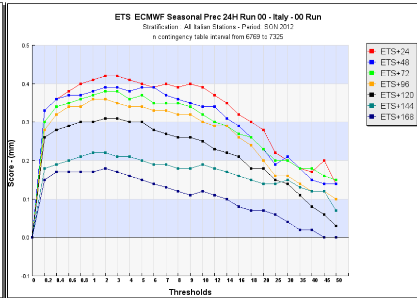
IFS Precipitation in 24 hours - ETS score
