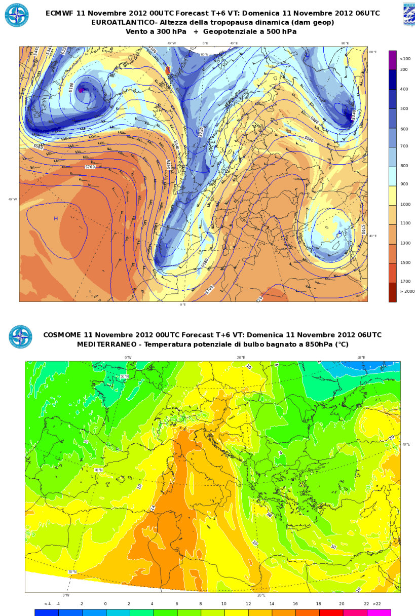
Figura 1 500 hPa Geopotential, Dynamic Tropopause and 300 hPa wind, showing an anomaly in upper air between Tunisia and Sicily (above); 850 hPa Wet Bulb Potential Temperature, showing a baroclinic area above Tyrrhenum Sea (below).
