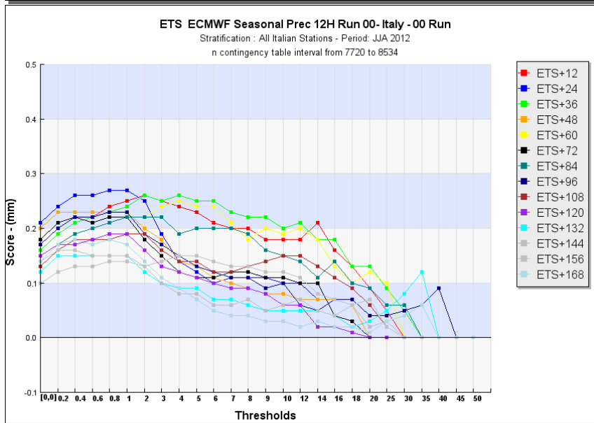
IFS Precipitation in 12 hours - ETS score
