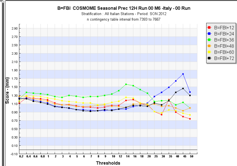
COSMO-ME Precipitation in 12 hours - FBI score
