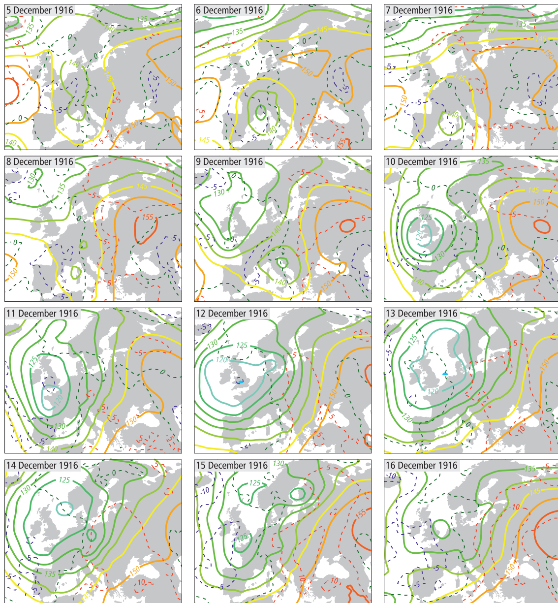
Figure 4 850 hPa geopotential height (solid contours; in decametres) and 850 hPa temperature anomaly with respect to the reference period 1961–90 (dashed contours; in °C) at 0000 UTC for each day from 5 to 16 December 1916 (ERA-20C).
