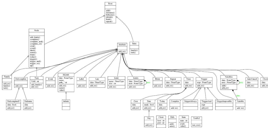
Class Diagram for module ecf.py .
