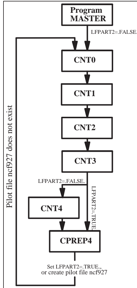
Figure 2.2 General mechanism of the so-called configuration (e)(e)927.
