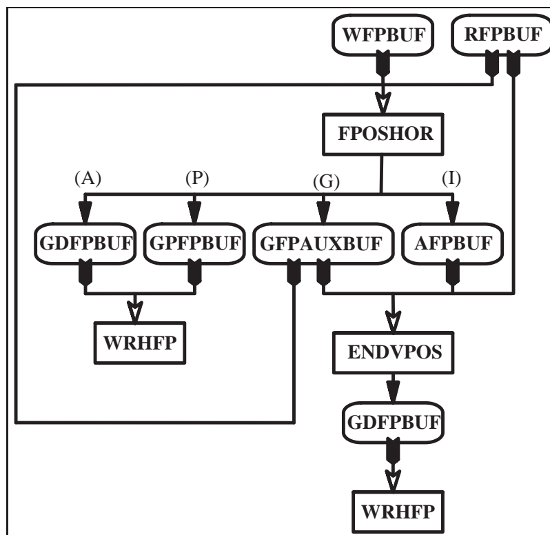
Figure 2.20 Fullpos buffers interactions in the horizontal interpolations.
