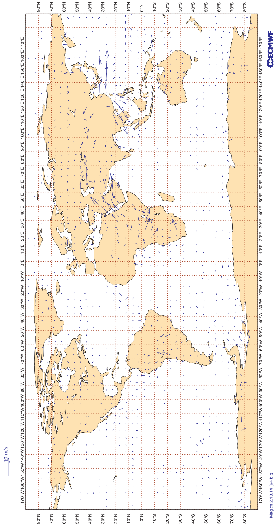
Figure 16 ECMWF Monitoring Statistics: May 2014 AMV Winds: 700-1000hPa Wind bias: Observation - FG
